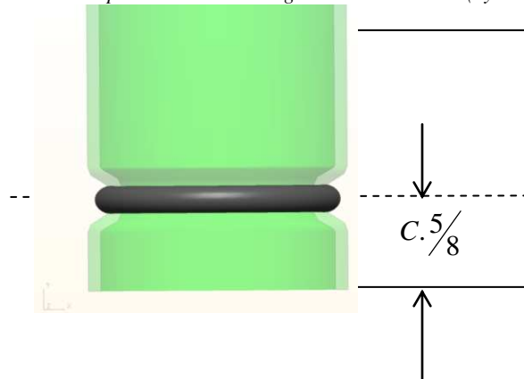
Figure No. 10. Spout Tube and O-ring Leak Free Feature (by Cruz, J.).
